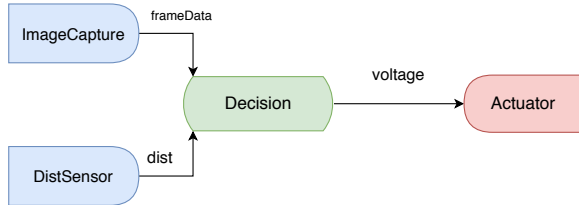
Figure 1: Example illustrating how a program looks like in the existing coordination language.
